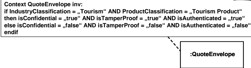
Figure 6 Constraint on an Information Envelope: Quote Envelope
