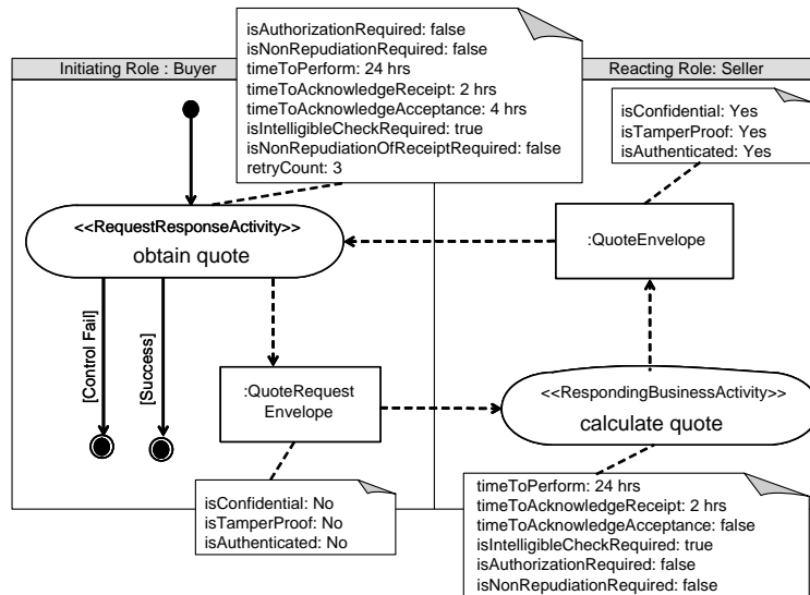
Figure 1. Business Transaction: Request for Quote
