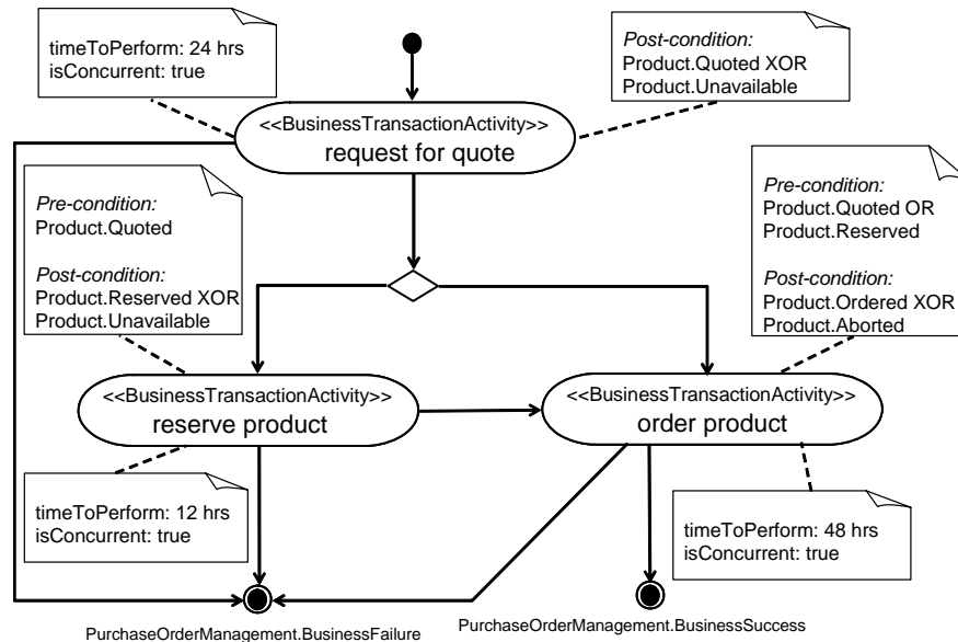
Figure 2. Business Collaboration Protocol: Purchase Order Management
